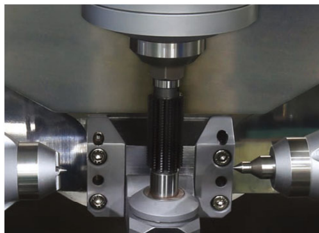
Hob Arbor Support Unit (滾刀支撐單元)
