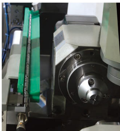
Feeder in Working Chamber (滾齒加工區的餵料裝置)
