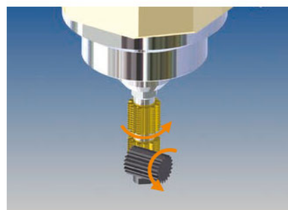
Two Hob Deburring (雙滾刀去毛邊裝置)
