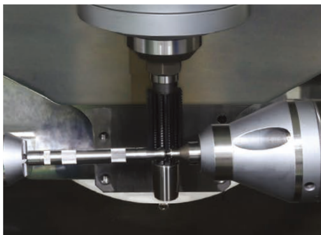
Dry Cutting / Skiving (乾式切削 / 熱處理後齒輪滾齒)
